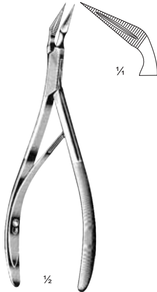
Ralk DC04-235-15 15 cm/6"
